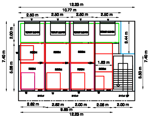
PRO. FIRST FLOOR PLAN (DWELLING HOUSE)
