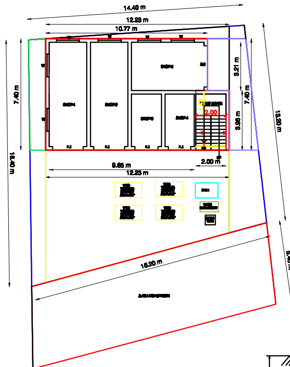
EXISTING GROUND FLOOR PLAN (COMMERCIAL)
