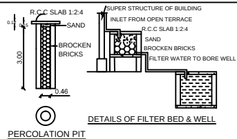
PERCOLATION PIT
