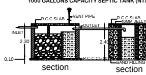
1000 GALLONS CAPACITY SEPTIC TANK (NTS)
