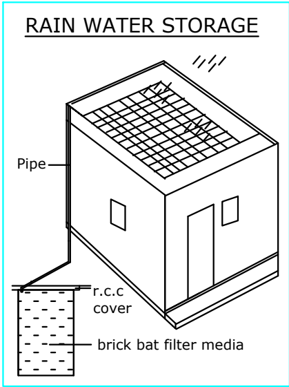
RAIN WATER STORAGE
