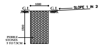
SECTION OF PEBBLE TRENCH SCALE: 1: = 100
