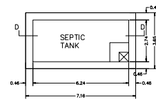
PLAN OF SEPTIC TANK SCALE 1" = 2'-0"
