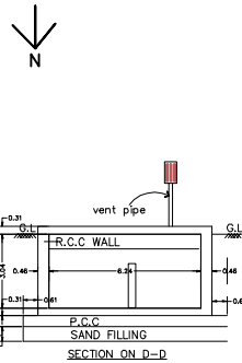
SECTION ON D-D
