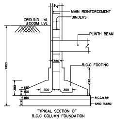
TYPICAL SECTION OF R.C.C. COLUMN FOUNDATION SCALE 1" = 2'-0"
