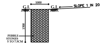
SECTION OF PEBBLE TRENCH SCALE: 1: = 100
