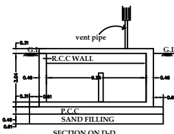
SECTION ON D-D
