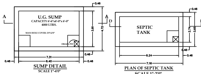
SUMP DETAIL
