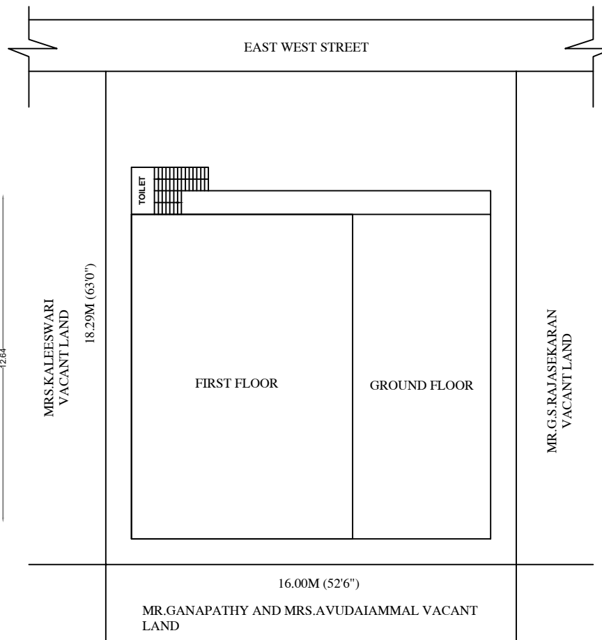
SITE PLAN
