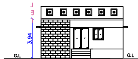
FRONT ELEVATION
