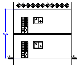
FRONT ELEVATION
