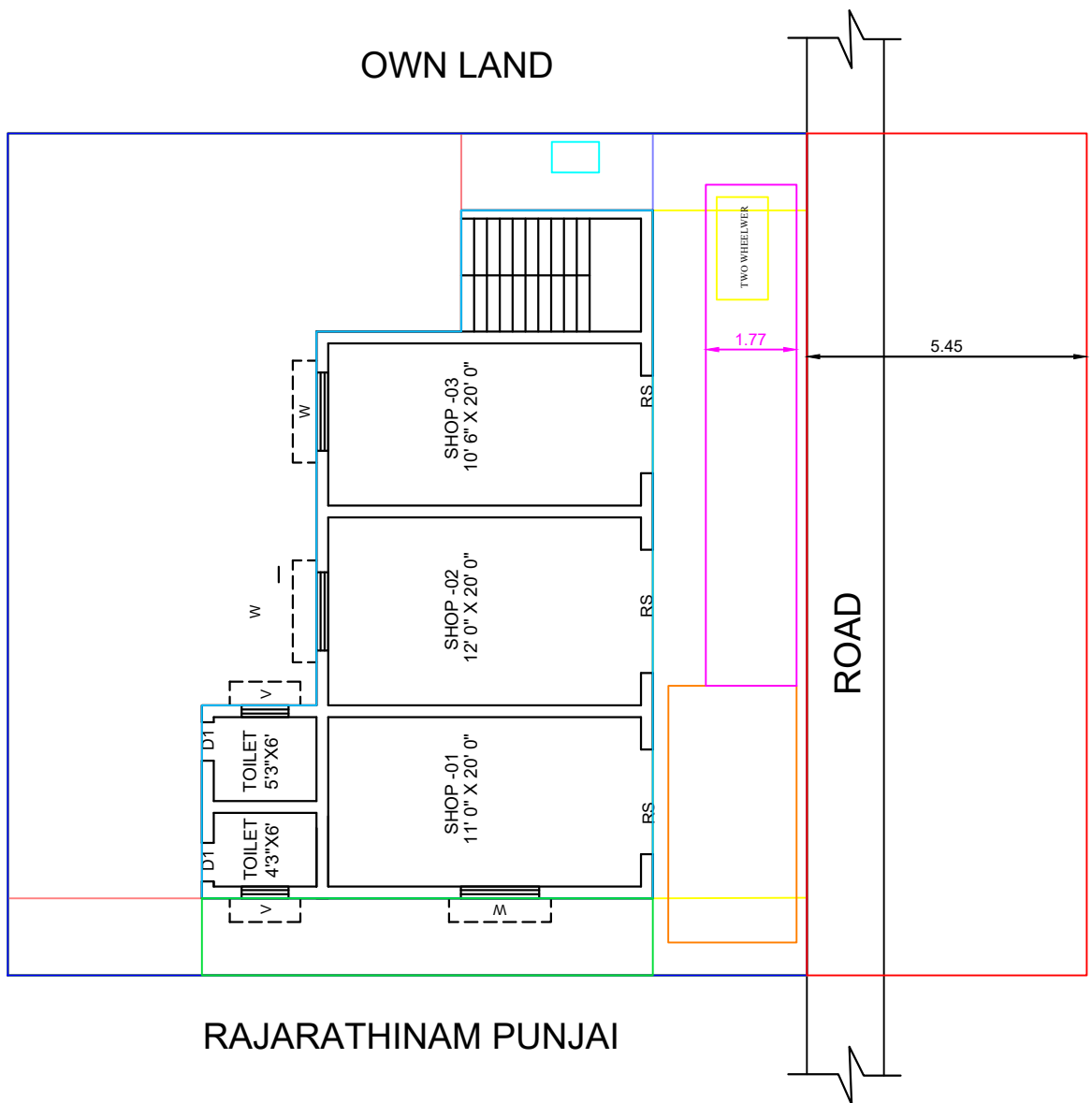
SITE PLAN
