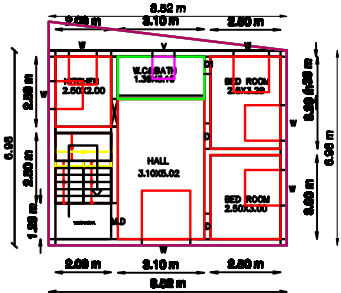
SECOND FLOOR PLAN (EXTENSION)
