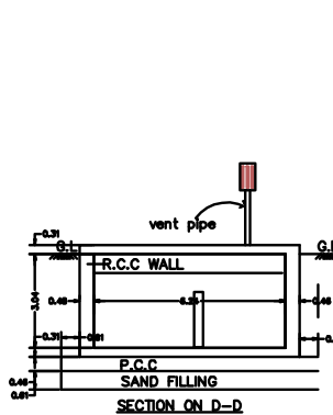
SECTION ON D-D
