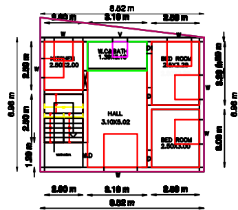
FIRST FLOOR PLAN (EXTENSION)
