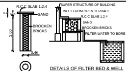
PERCOLATION PIT
