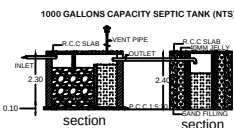
1000 GALLONS CAPACITY SEPTIC TANK (NTS)
