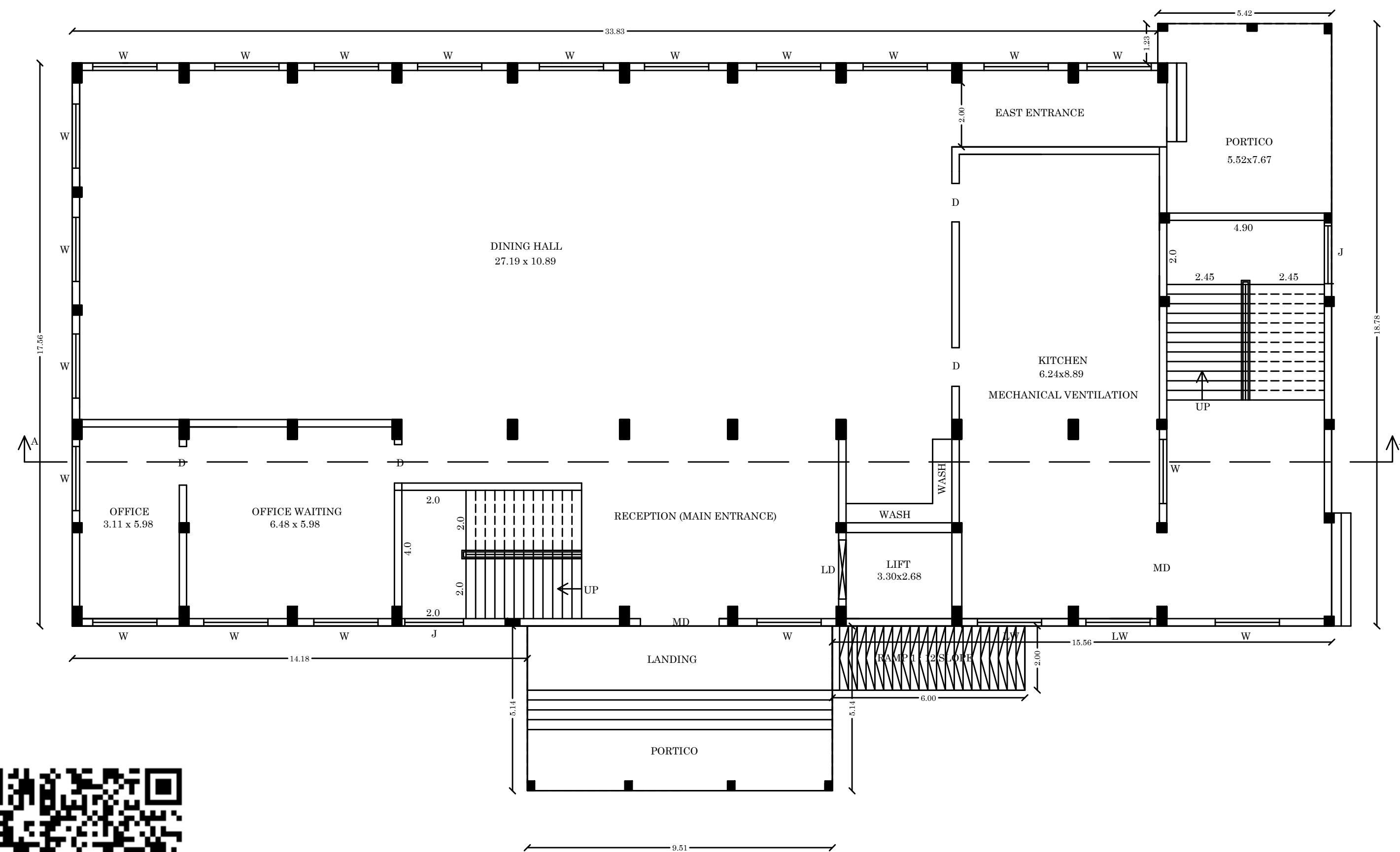
GROUND FLOOR PLAN Block -1
