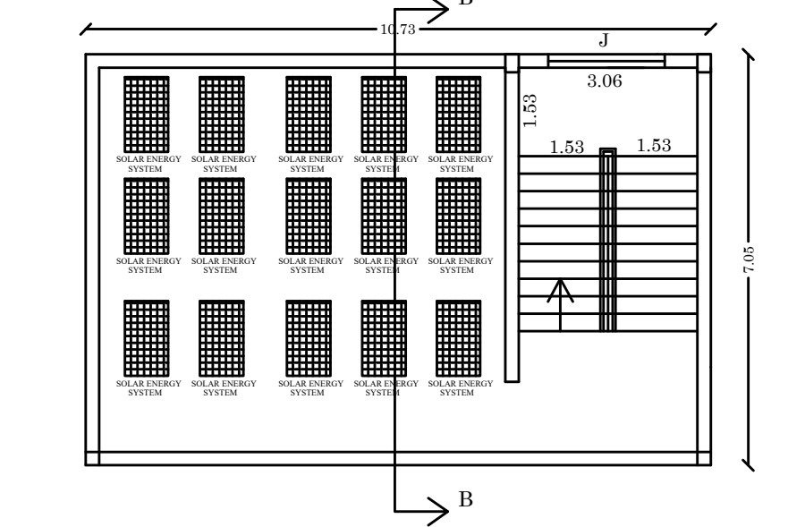
TERRACE FLOOR PLAN Block -2
