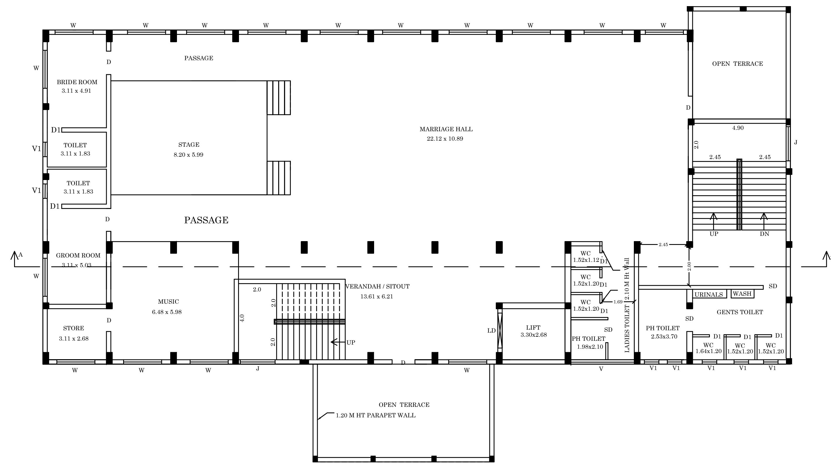
FIRST FLOOR PLAN Block -1
