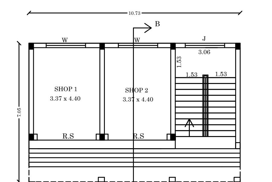
GROUND FLOOR PLAN Block -2
