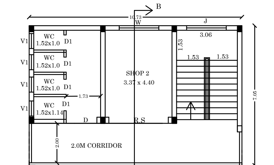
SECOND FLOOR PLAN Block -2
