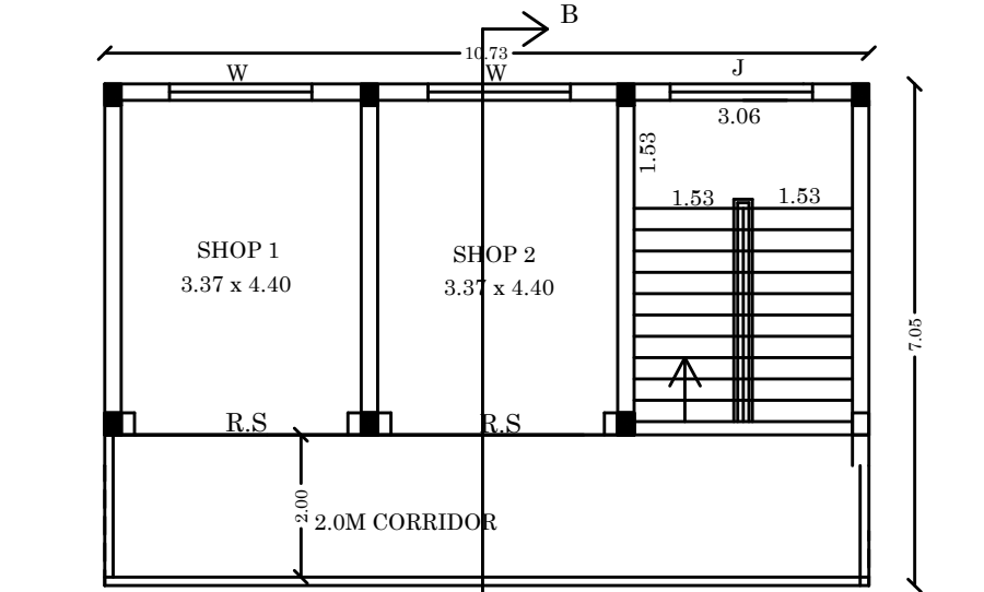
FIRST FLOOR PLAN Block -2
