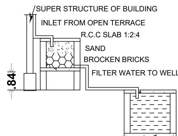
RAINWATER HARVESTING
