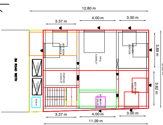
GROUND FLOOR PLAN (EXISTING) (EXTENSION)
