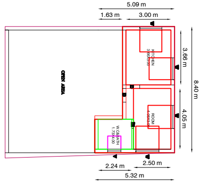
SECOND FLOOR PLAN (EXTENSION)
