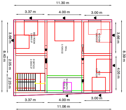
FIRST FLOOR PLAN (EXTENSION)
