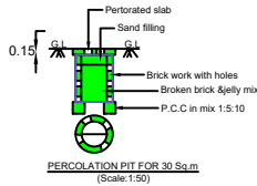
PERCOLATION PIT FOR 30 Sq.m (Scale: 1:50)
