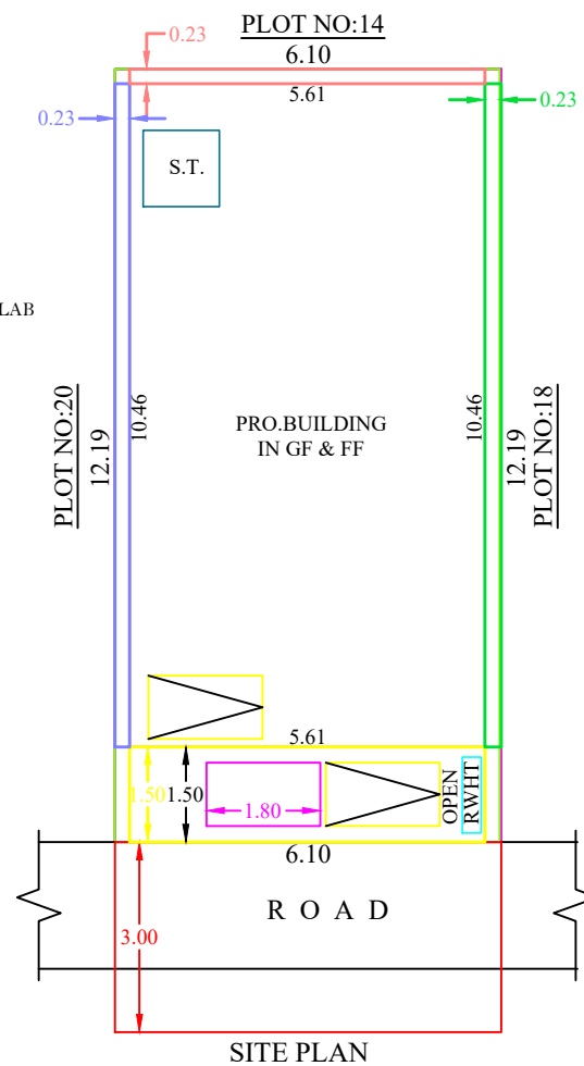
SITE PLAN
