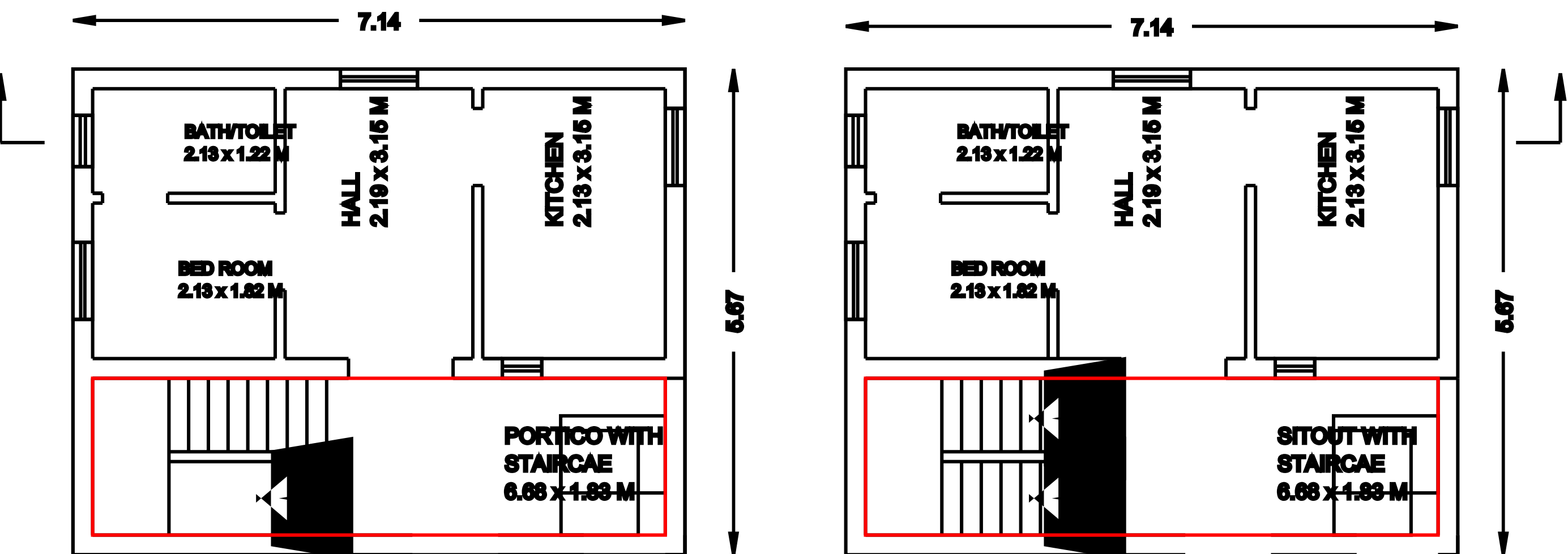
PROPOSED GROUND FLOOR PLAN
