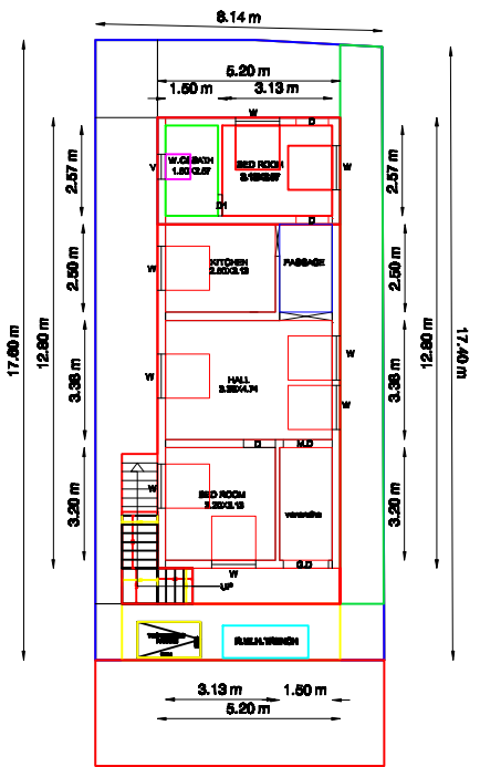
EXISTING & EXTENSION (PART) GROUND FLOOR PLAN
