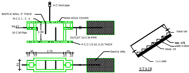
SEPTIC TANK AND TRENCH
