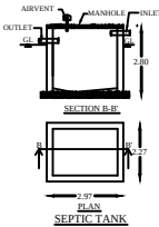
PLAN SEPTIC TANK
