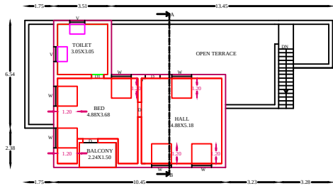
FF PLAN
