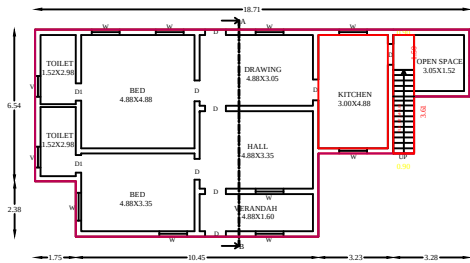
GF PLAN
