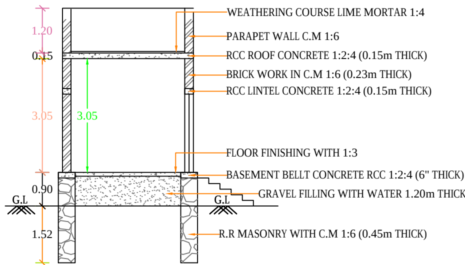
SECTION PLAN
