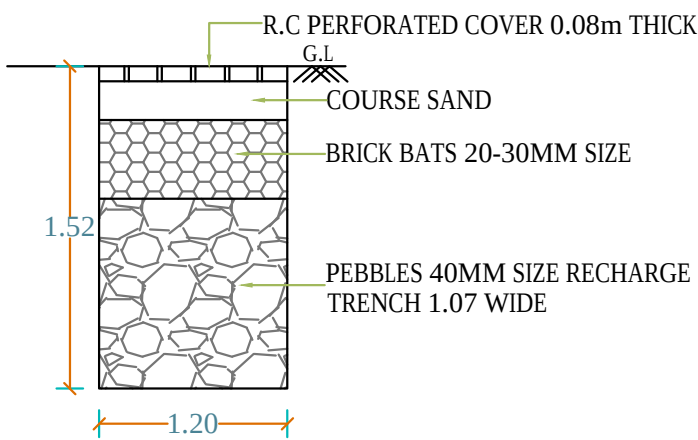
SECTIONAL VIEW OF RAIN WATER HARVESTING TRENCH
