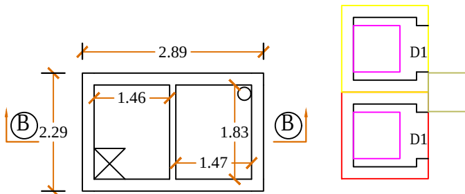
SEPTIC TANK
