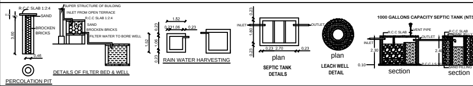
PERCOLATION PIT
