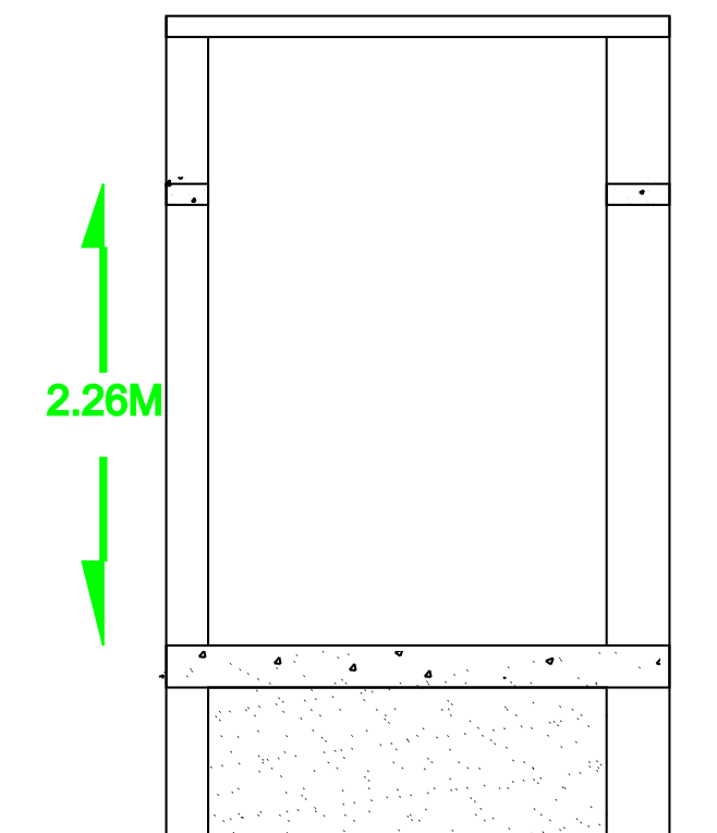
EAST FACE ELEVATION
