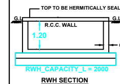
RW SECTION
