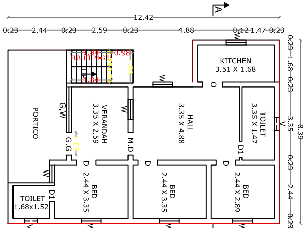
GROUND FLOOR PLAN (EXG. BUILDING)
