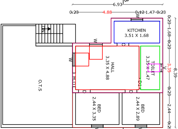
FIRST FLOOR PLAN (EXG. & PRO. BUILDING)
