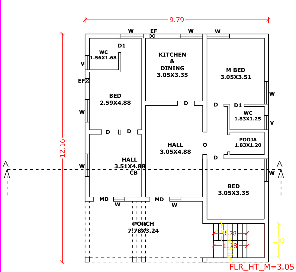
GROUND FLOOR PLAN (EXG. BUILDING)
