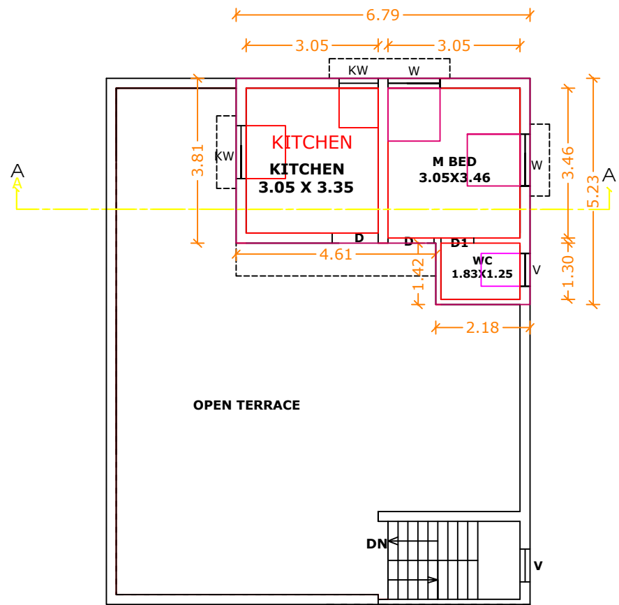
FIRST FLOOR PLAN (PRO. BUILDING)
