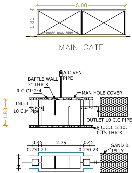
SEPTIC TANK AND TRECH
