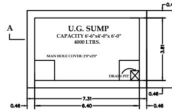
SUMP DETAIL
