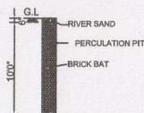
PERCULATION PIT
