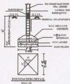
FOUNDATION DETAIL [DETAIL: 1/8"]
