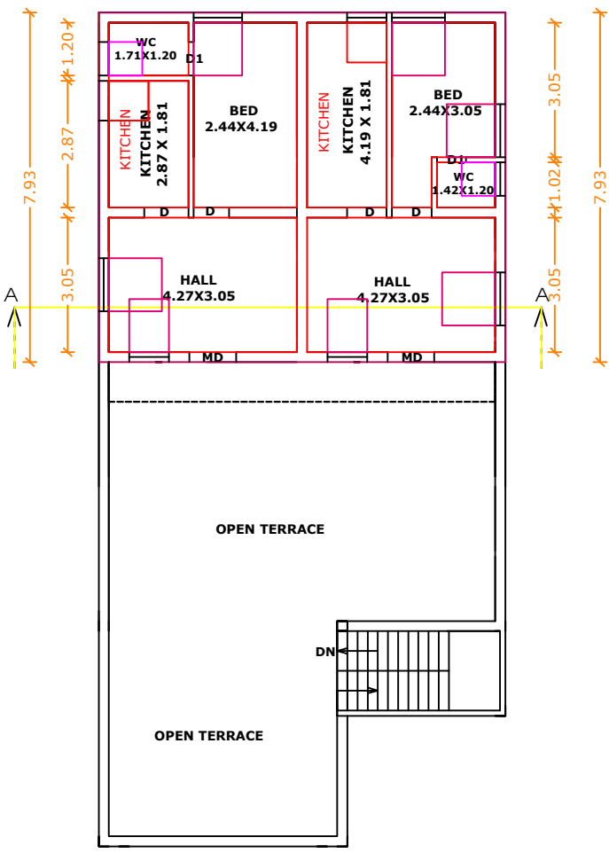
FIRST FLOOR PLAN (PRO. BUILDING)
