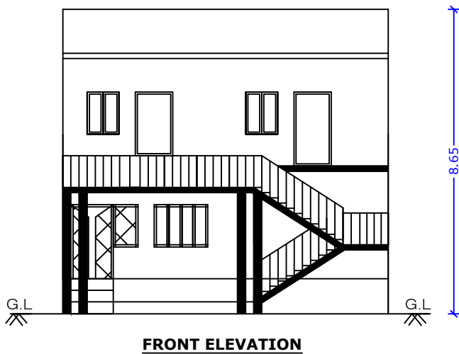
FRONT ELEVATION
