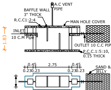
SEPTIC TANK AND TRECH
