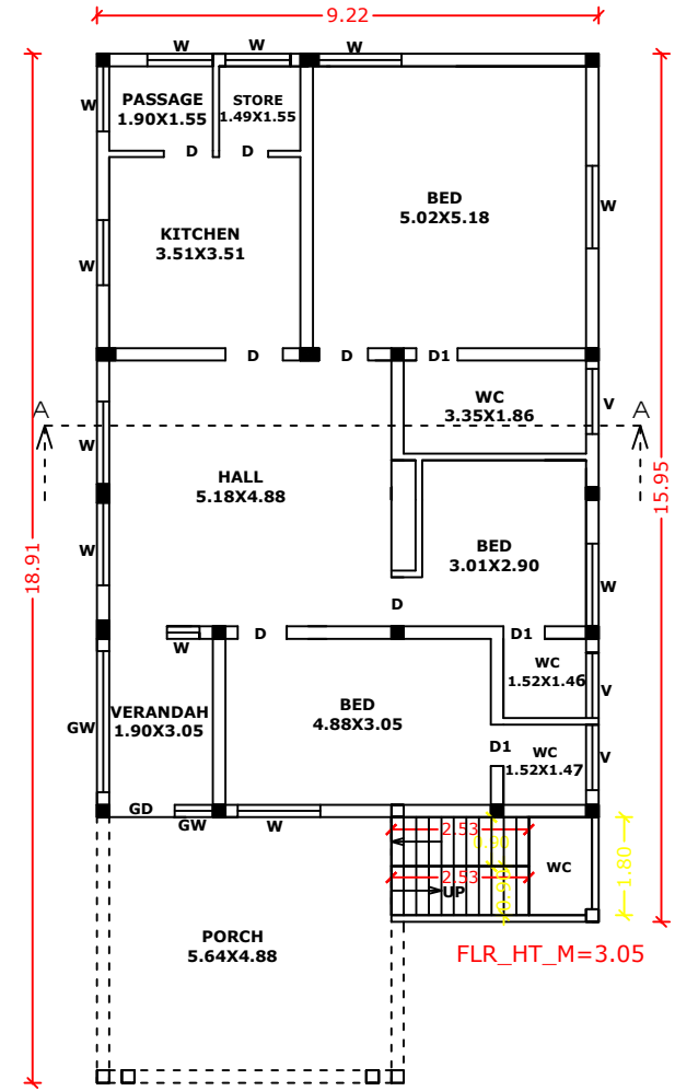
GROUND FLOOR PLAN (EXG. BUILDING)
