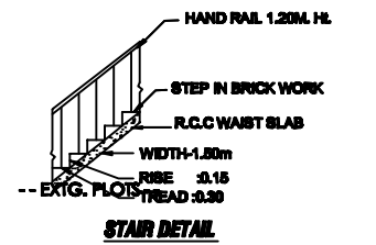
STAIR DETAIL
