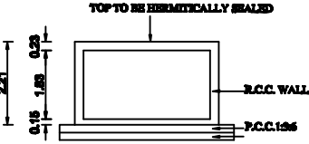
SECTION ON "U.G.SUMP"
