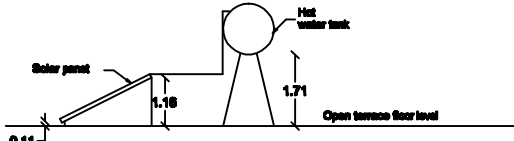
SIDE ELEVATION
