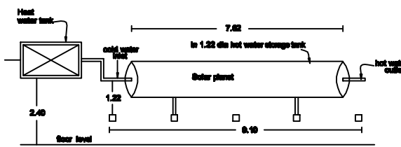
SOLAR WATER HEATER PLANT
