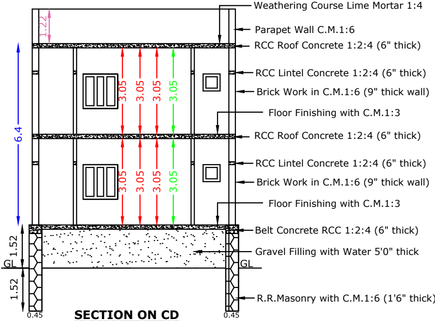
SECTION ON CD
