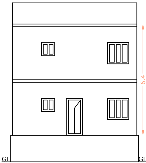
FRONT ELEVATION (RESIDENTIAL PORTION)
