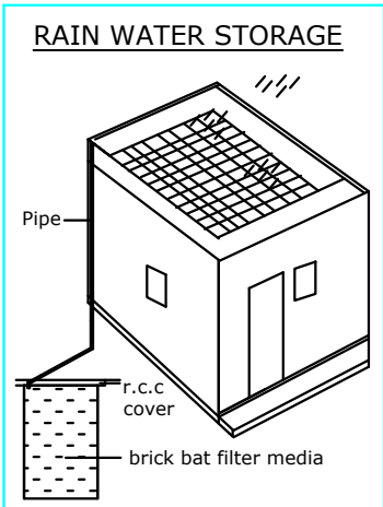
RWH_CAPACITY_L = 2000
