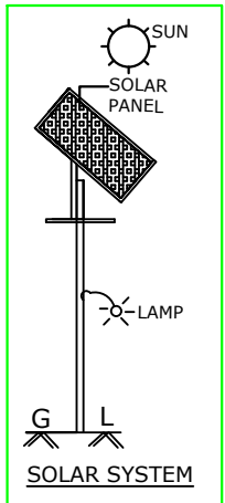
SOLAR SYSTEM
