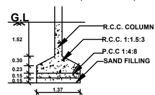
FOUNDATION DETAILS ( NOT TO SCALE)
