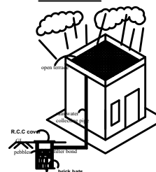
RAIN WATER HARVESTING ARRANGEMENT
