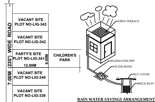
SITE PLAN SCALE:1CM=4M
