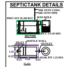
PLAN INFORMATION
