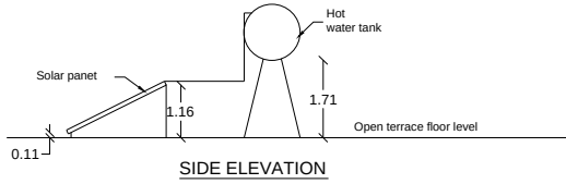
SIDE ELEVATION
