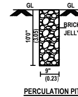
PERCULATION PIT
