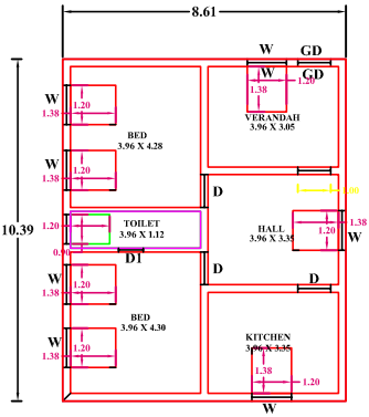
PLAN AT FIRST FLOOR
