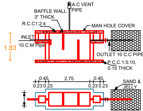
SEPTIC TANK AND TRECH
