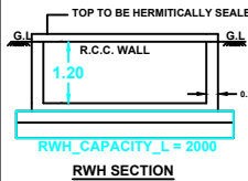
RWHS SECTION
