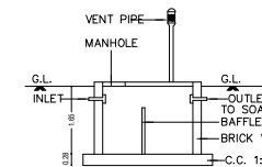
SECTION OF SEPT. TANK
