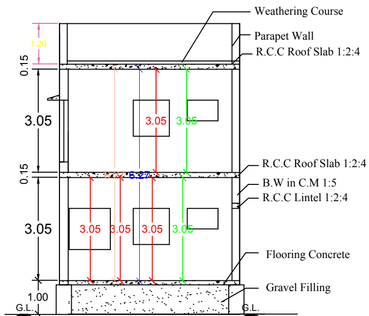
CROSS SECTION - AA
