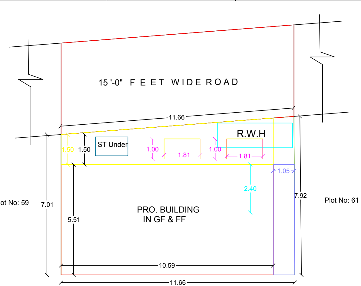
SITE PLAN
