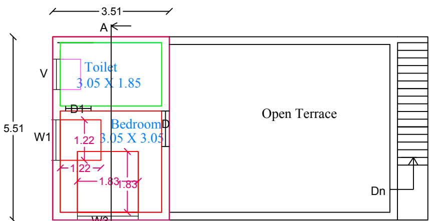
PRO FIRST FLOOR PLAN
