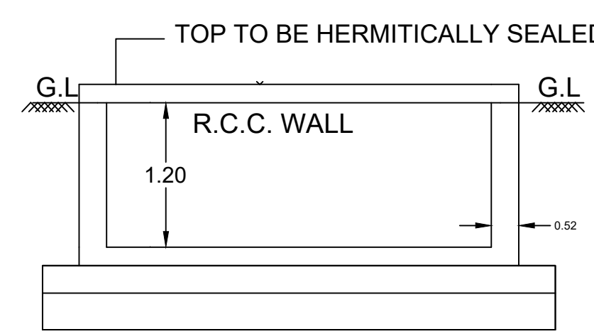
RWH_CAPACITY_L = 2000 RWH SECTION
