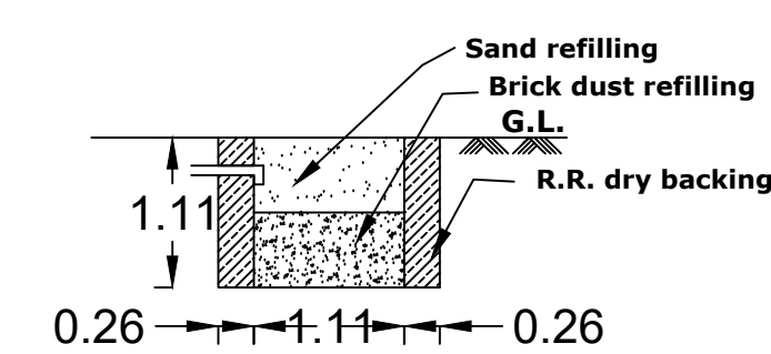
DETAILS OF RAIN WATER HARVESTING
