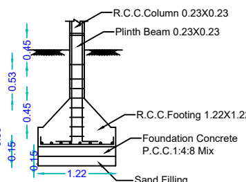
DETAILS OF COLUMN FOOTING
