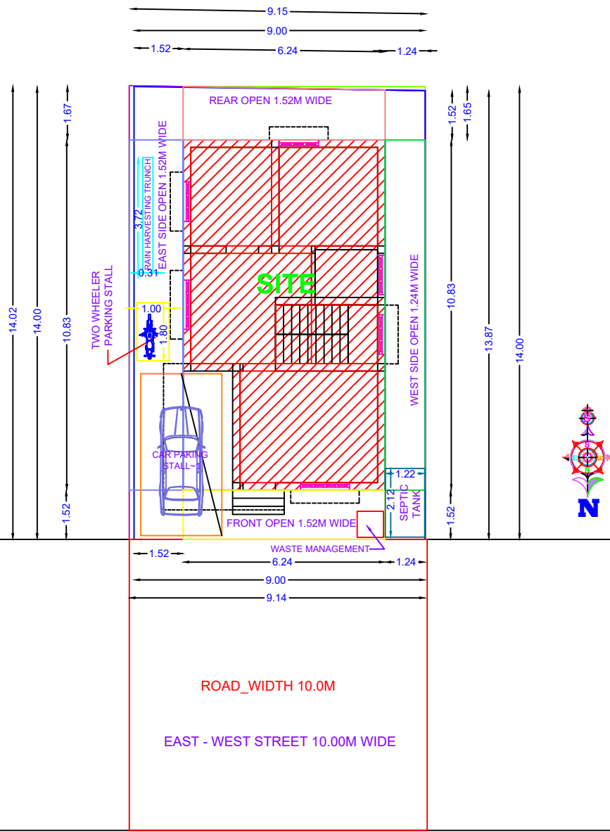
SITE PLAN
