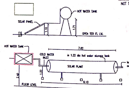
SOLAR WATER HEATER PLANT DETAILS
