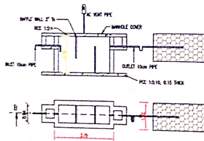
SEPTIC TANK AND TRENCH & U TRAP
