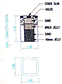
RAIN WATER COLLECTION TANK
