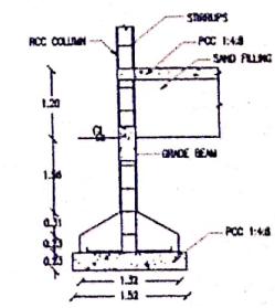
COLUMN DETAILS
