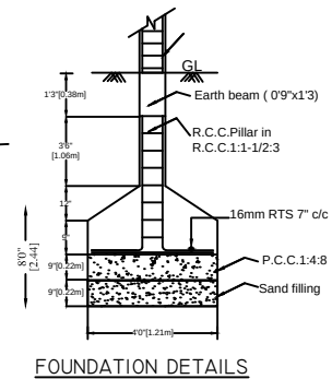
FOUNDATION DETAILS
