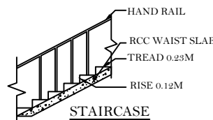
STAIRCASE
