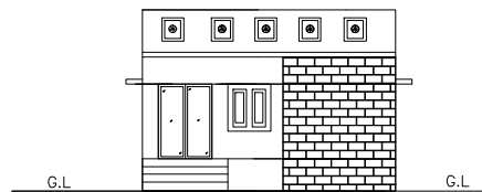
FRONT ELEVATION
