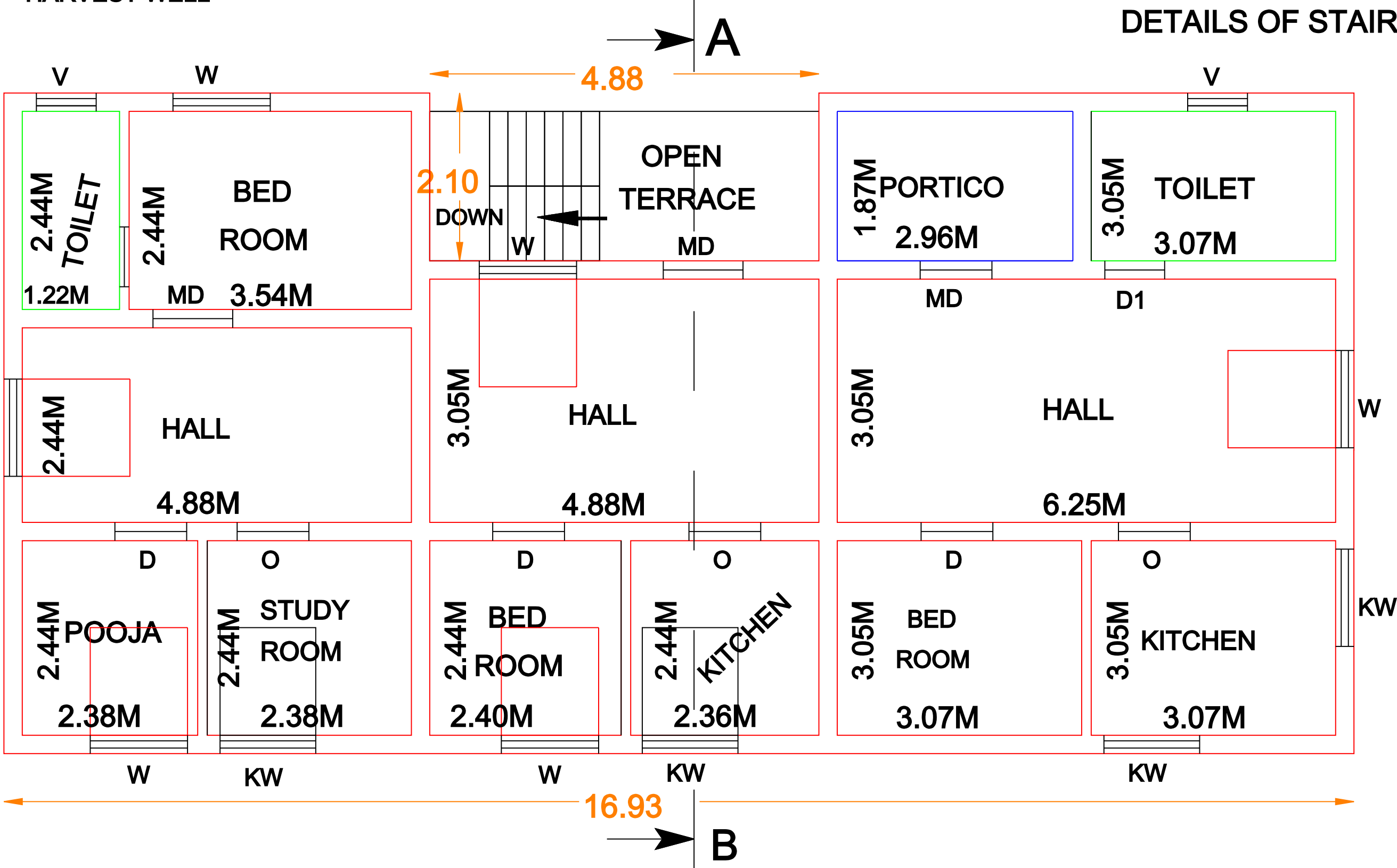
DETAILS OF STAIRCASE
