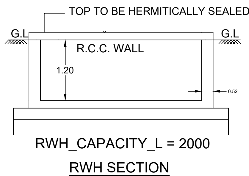
RWH SECTION
