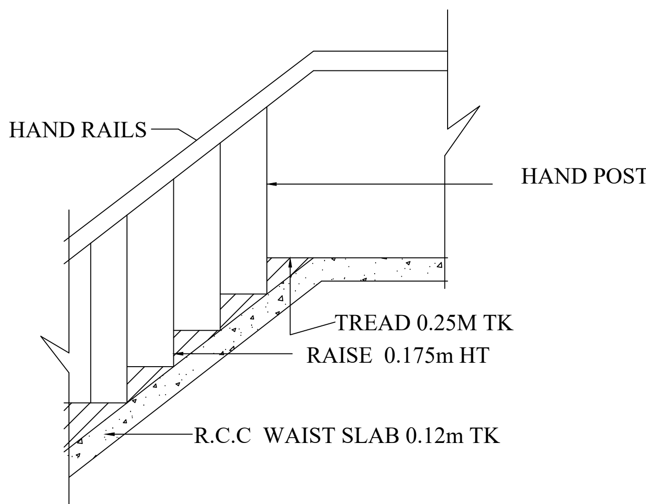
STAIRCASE DETAILS
